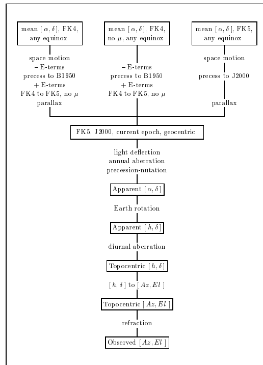
Figure 1: Relationship Between Celestial Coordinates
