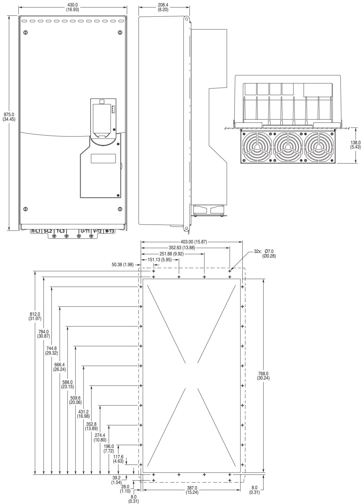
Figure A.22 Flange Mount, Frame 7
