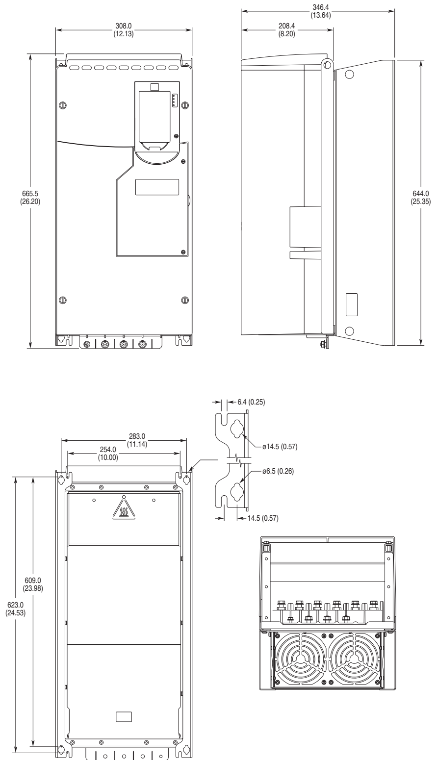
Figure A.17 IP00, NEMA/UL Open Type, Frame 6
