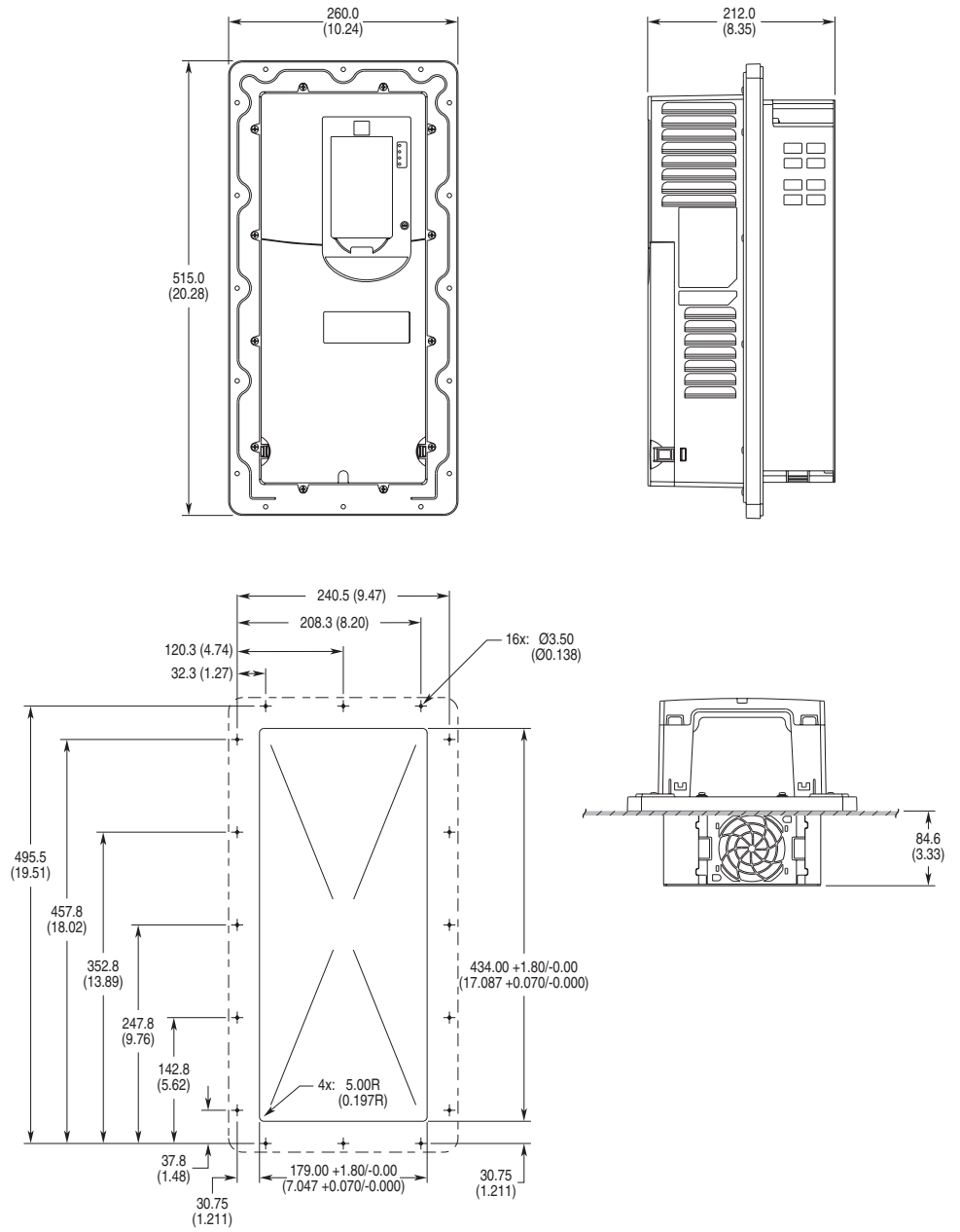
Figure A.6 Flange Mount, Frame 3
