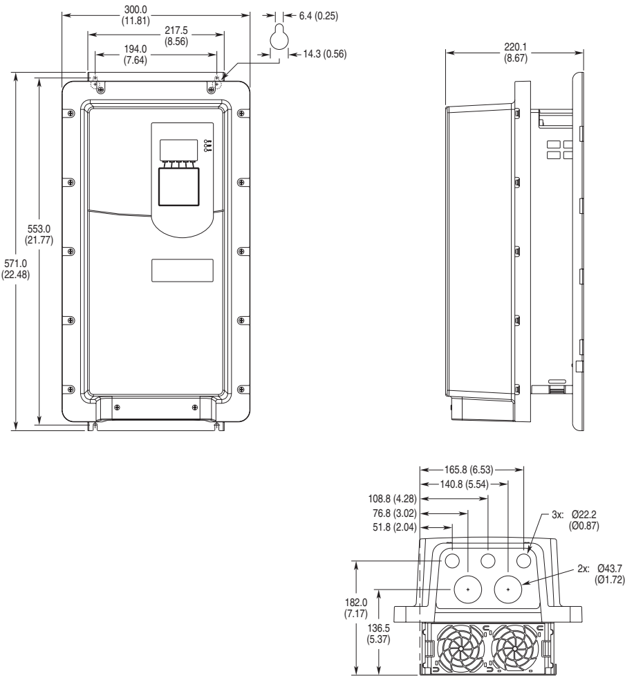
Figure A.10 IP54, NEMA/UL Type 12, Frame 4
