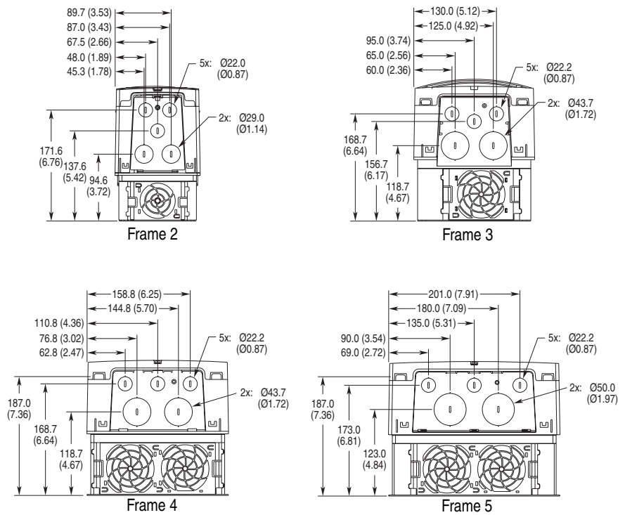
Figure A.15 NEMA/UL Type 1 Frames 2...5 Bottom View Dimensions
