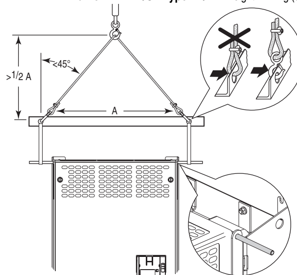
Figure 1.2 Frame 7 Open Type and Flange Mount: Weight: 72.6...108.9 kg (160...240 lb) Frame 6 NEMA/UL Type 4X/12: Weight: 90.7 kg (200 lb) Frame 7 NEMA/UL Type 4X/12: Weight: 171 kg (377 lb)
