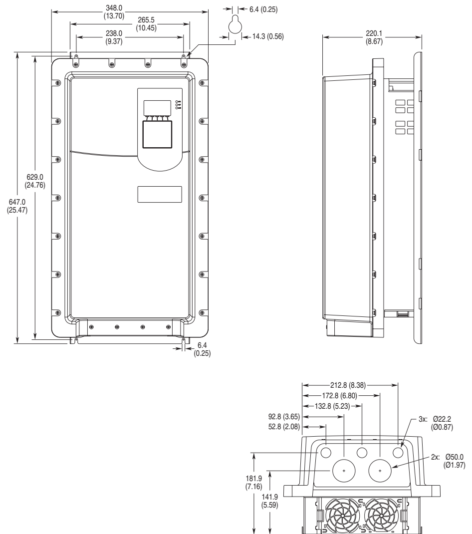
Figure A.13 IP54, NEMA/UL Type 12, Frame 5
