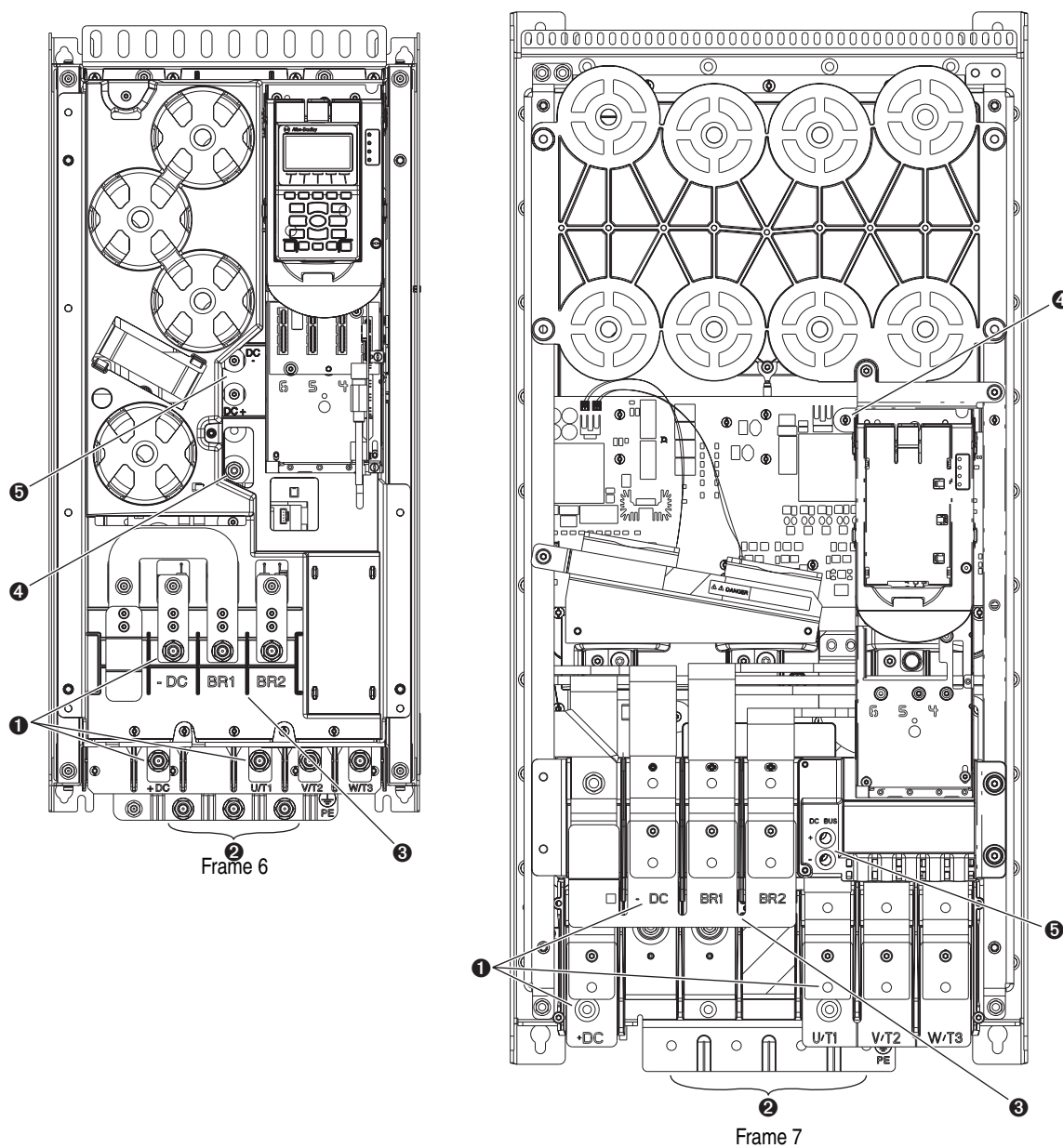
Figure 1.11 Common Bus Terminal Block Location and Termination Points (continued)
