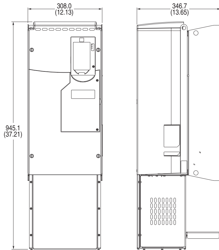
Figure A.19 NEMA/UL Type 1 Kit Frame 6
