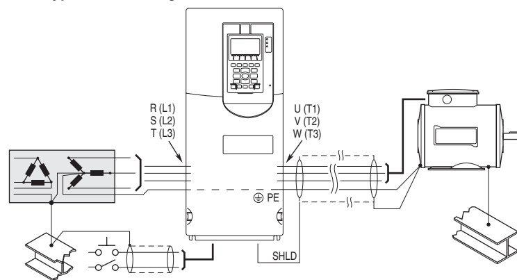
Figure 1.7 Typical Grounding
