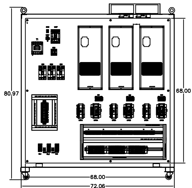
PANEL LAYOUT
