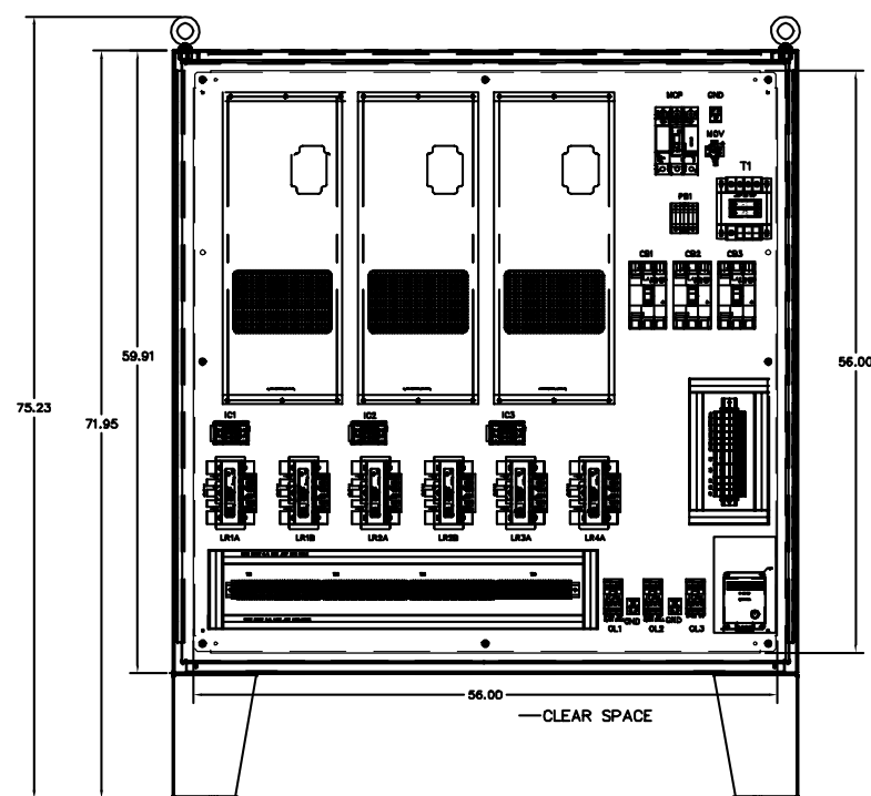
PANEL LAYOUT
