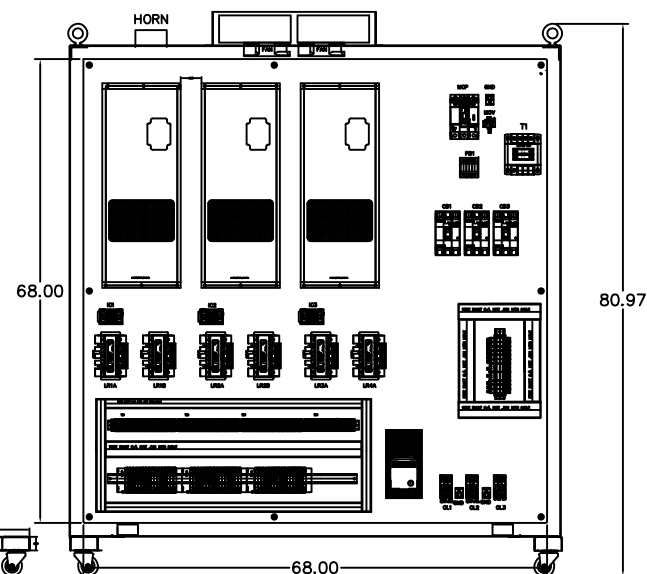
PANEL LAYOUT
