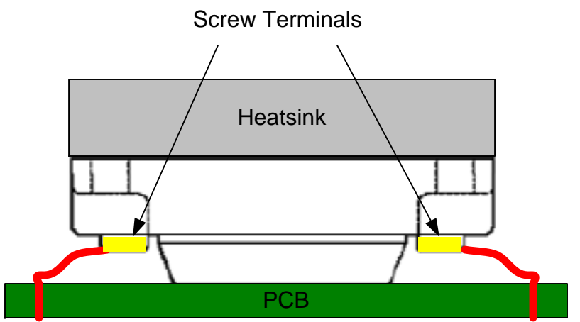
Solid State Relay Mounting & Wiring
