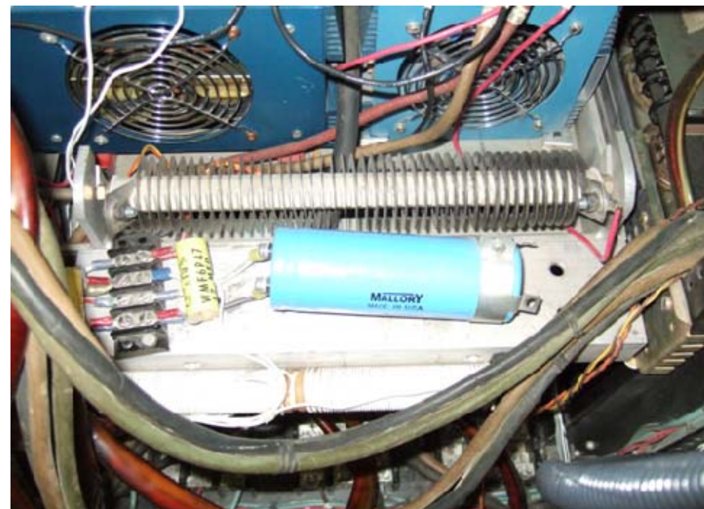
Dome amp power supply 1.5 ohm resistor
