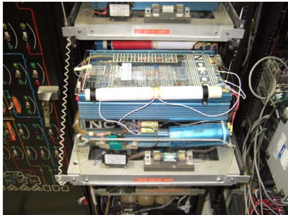
Dome East servo amp and external components.
