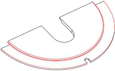
ISOVIEW 2 SCALE 1:2
