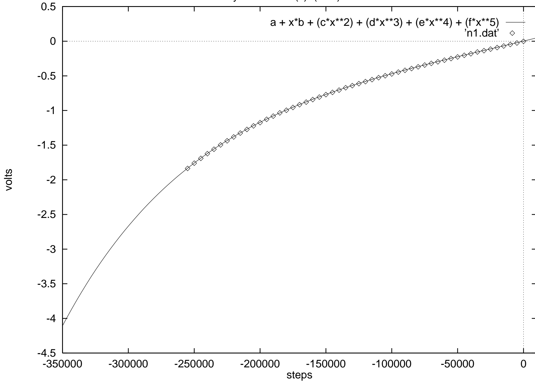
Array Focus v = f(s) (cold) - 7/23/99
