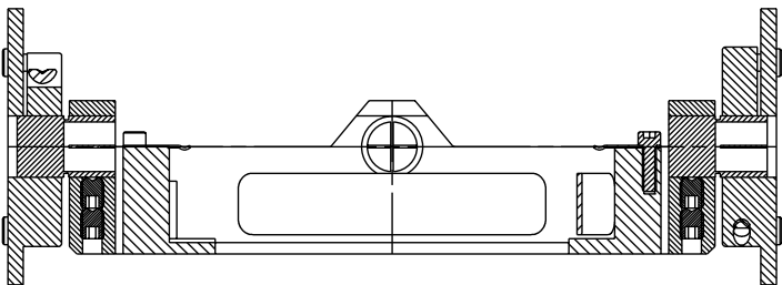
SECTION B-B: SCALE 1 : 1
