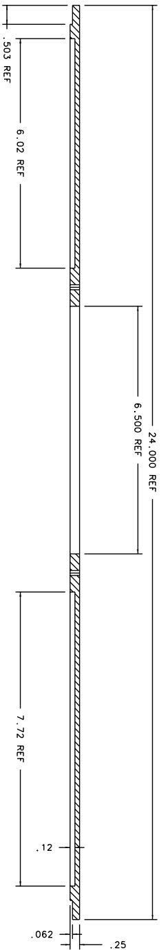
SECTION B-B: SCALE 1:2
