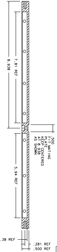
SECTION B-B: SCALE 1:2
