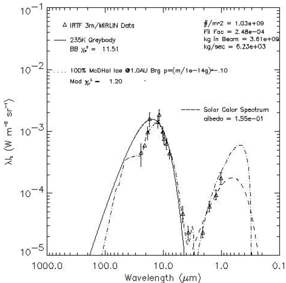
Figure 2. Spectral energy distributions of comet C/1999 S4 (LINEAR) (triangles) as observed on 17 June 2000 using a 7" radius aperture. Dashed curve - solar spectrum normalized to LS4 observation at 1.25 \mu\text{m} . Solid curve - modified greybody fit to the mid-IR data. The best-fit greybody temperature is 38 K cooler than the local equilibrium temperature. From 12 to 25 \mu\text{m} , there is a strong absorption feature present due to water ice. Dash-dash-dotted Curve - best-fit fractal particle model with 100% water ice and a comet Halley particle size distribution.
